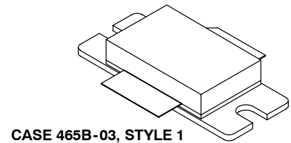
CASE 465B-03, STYLE 1 NI-880 MRF6S24140HR3
